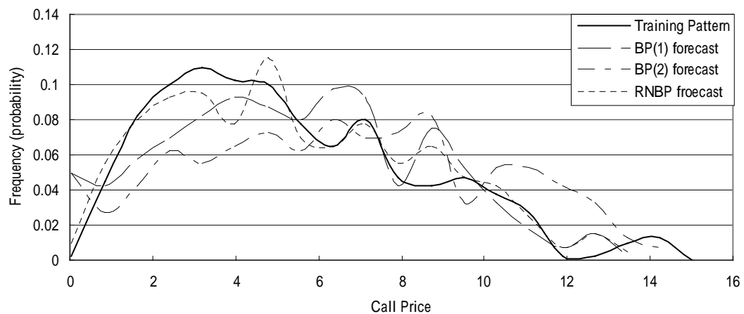
Figure 6 The frequency distribution in the out-of-the-money experiment
